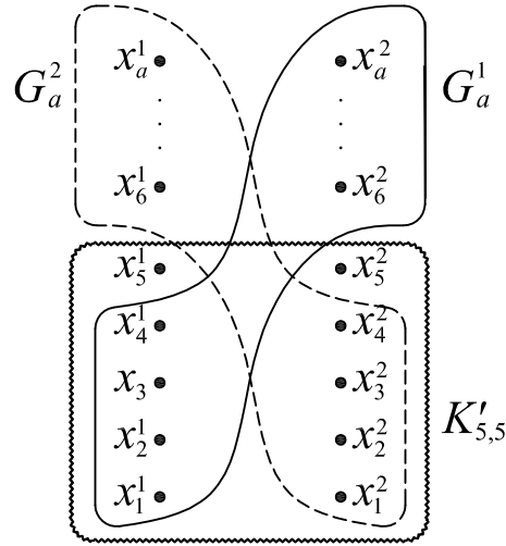
Figure 3: The graph H_a
