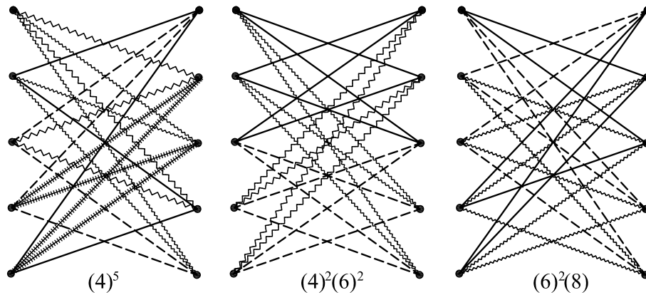
Figure 1: K'_{5,5} -realizations of three sequences
