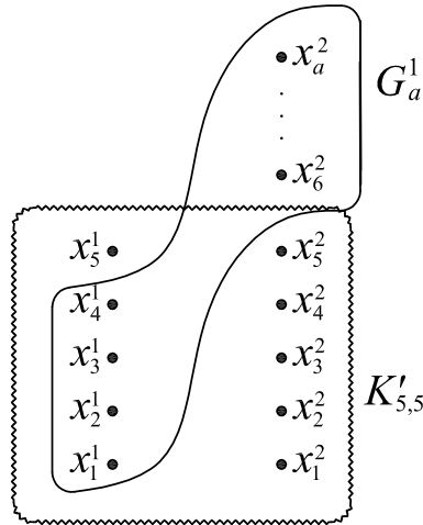
Figure 2: The graph G_a
