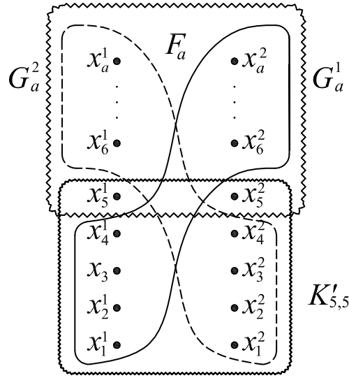
Figure 4: The graph K'_{a,a}
